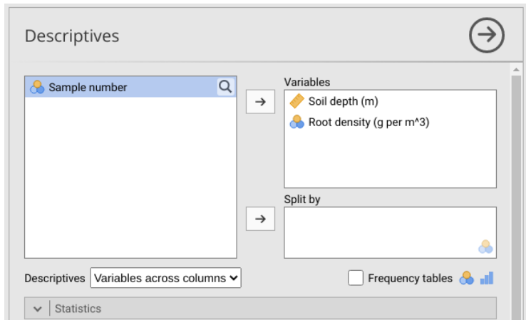
Figure 3: Jamovi input for testing normality.
