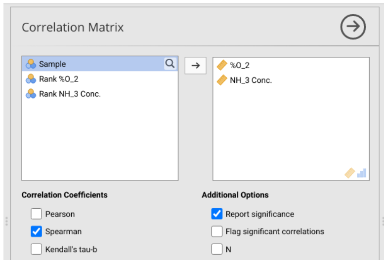
Figure 8: Jamovi box showing how to run a test of the Spearman rank correlation coefficient.
