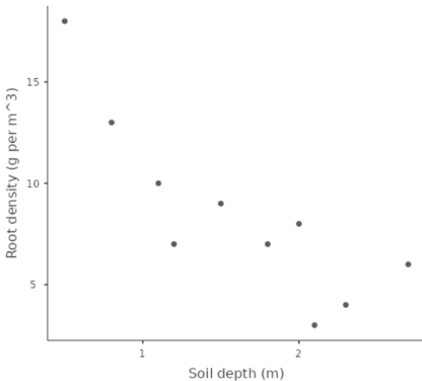
Figure 5: Jamovi output of a scatterplot for Soil Depth vs Root Density
