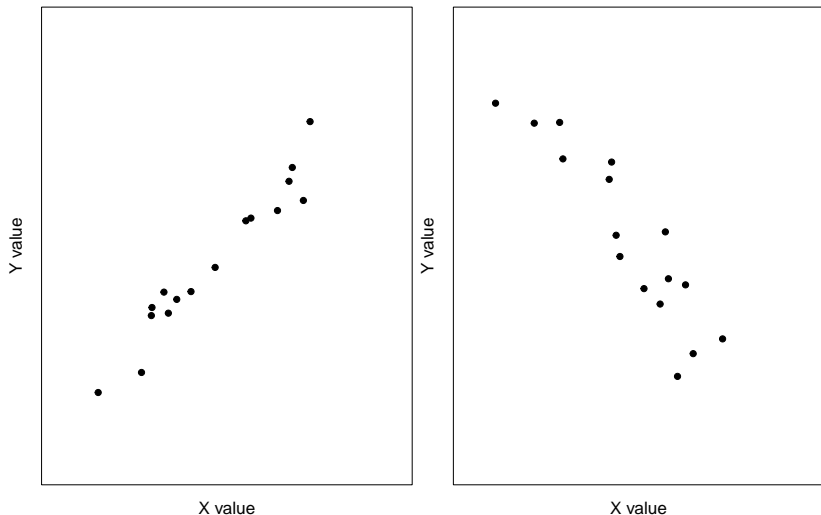
Figure 1: Variables illustrating a positive (left) and negative correlation
